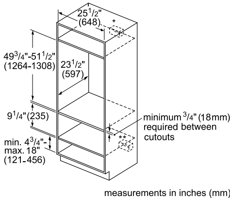
Standard Installation 27" Double Oven over Warming Drawer
