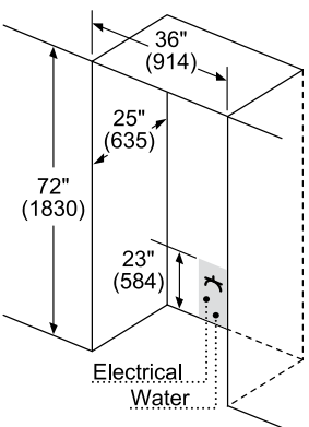
36" Freestanding Installation
