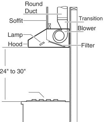
Vertical discharge
