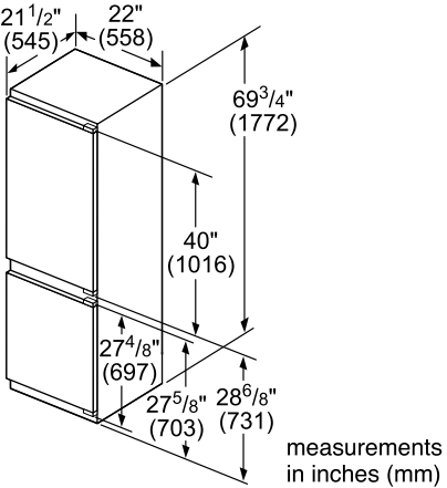
B09IB81NSP Dimensions
