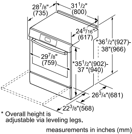
Electric Range Dimensions
