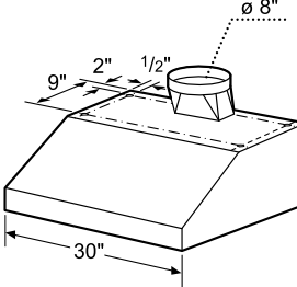
800 Series 30" DPH30652UC Under-Cabinet Hood
