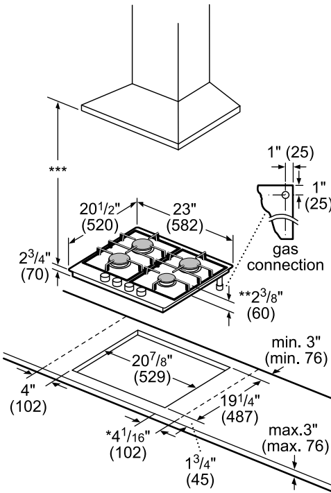
24" Cooktop and Cutout Dimensions
