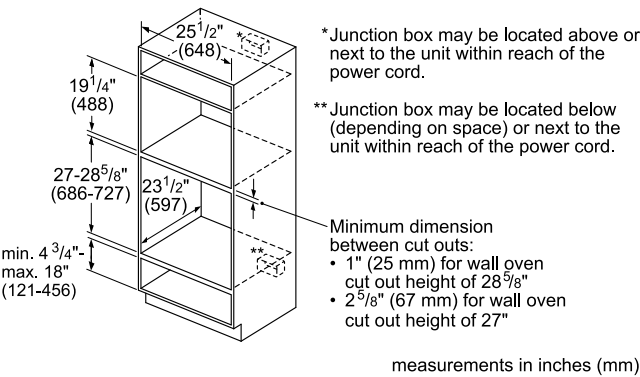
Standard Installation 27" Speed Oven or Microwave over Single Oven
