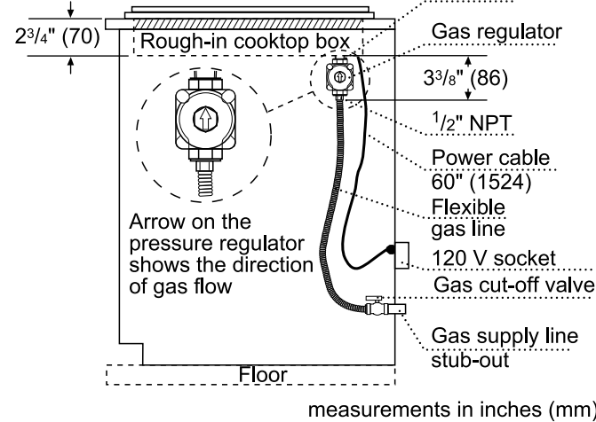
24" Cooktop Gas Location
