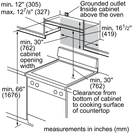
300 Series Cutout and Clearances
