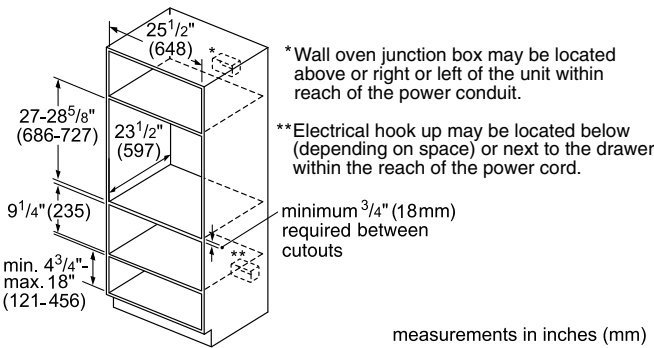
Standard Installation 27" Single Oven over Warming Drawer
