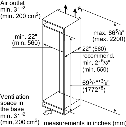
B09IB81NSP Installation
