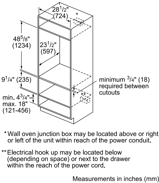
Standard Installation Combination Oven over Storage or Warming Drawer
