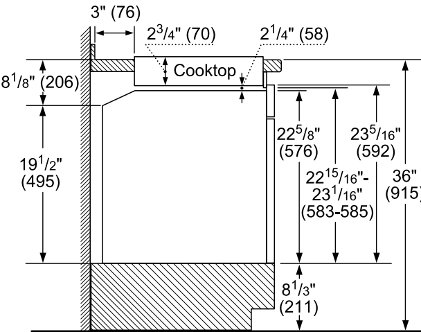
24" Cooktop Installation Above Wall Oven
