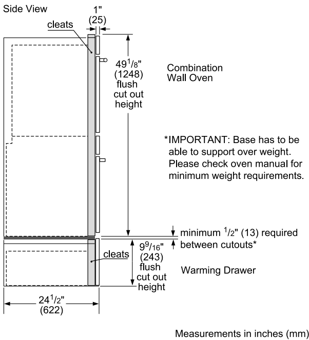
Flush Installation Combination Oven over Storage or Warming Drawer
