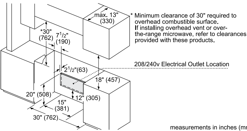
Induction Range Installation
