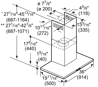
36" HCB56651UC Box Canopy Chimney Hood
