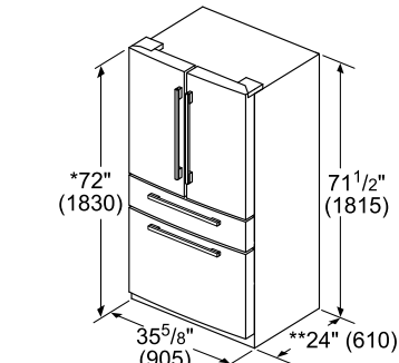
B36CL80SNS Dimensions
