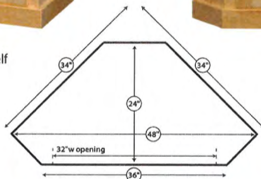
VR550 Corner TV Stand 48"w x 28"h x 24"d Requires 34" of wall space on both sides of unit Opening in front is 32"w
